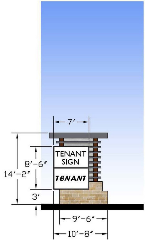
2 - 4'-3" X 7' PANELS EACH SIDE TENANT MONUMENT 59.5 SF Each Side
