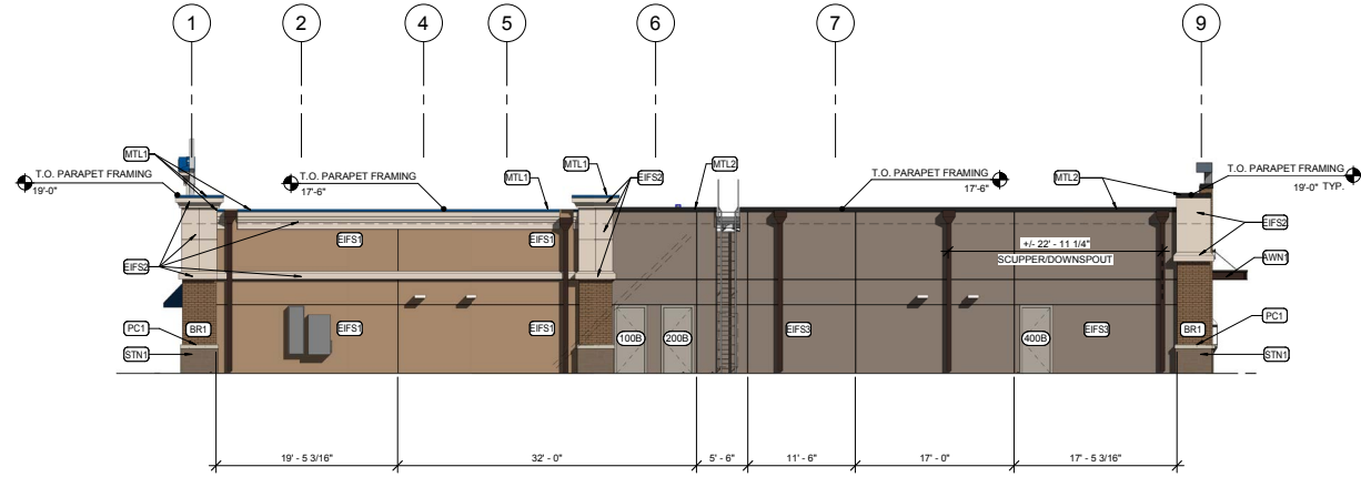
3 RENDERED REAR/SOUTH ELEVATION
