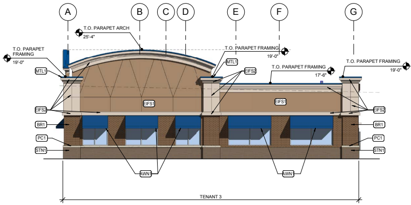
4 RENDERED WEST ELEVATION
